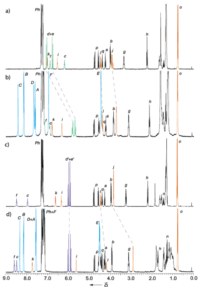
Figure 1. 1 H NMR spectra (400 MHz in CDCl 3 at 298 K) of (a) fumaramide thread E-2 , (b) fumaramide rotaxane E-1 , (c) maleamide thread Z-2 , (d) maleamide rotaxane Z-1 . The assignments correspond to the lettering shown in Scheme 1.
